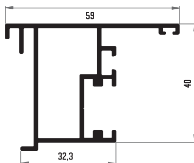
208 INVERSOR CENTRAL
